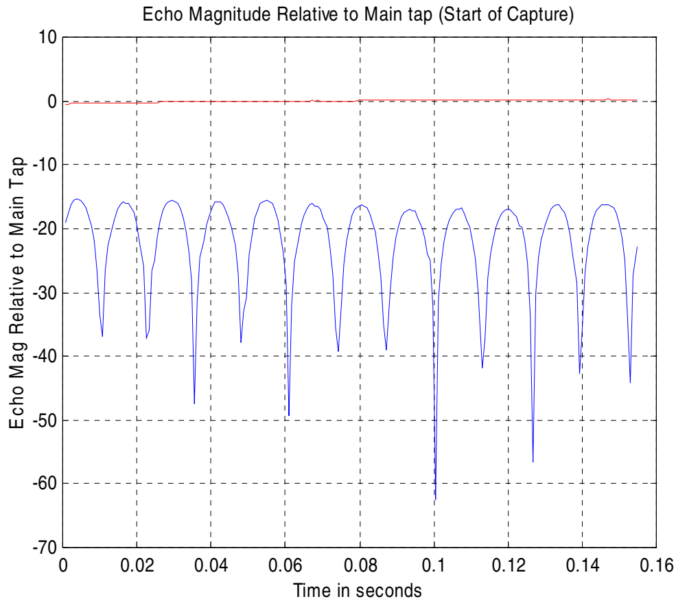
Figure B.12 Echo Magnitude for the 1.75 \mu\text{s} echo relative to the main path at the beginning of the capture at indoor site WAS-49/36/01. The echo magnitude is -15 dB relative to the main path. The Doppler frequency is 40 Hz.
