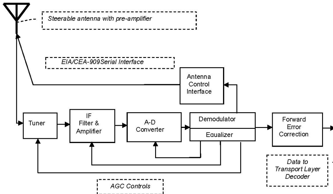
Figure 3.2 Digital television receiver front-end subsystem block diagram.
