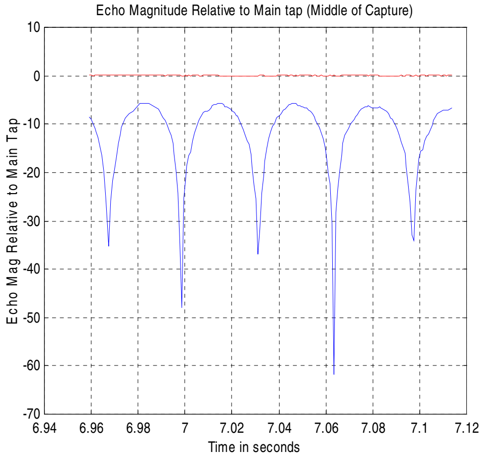
Figure B.10 The 11 \mu\text{s} echo magnitude 6.9 seconds into the capture at indoor site WAS-32/39/01. Doppler frequency is 17 Hz.
