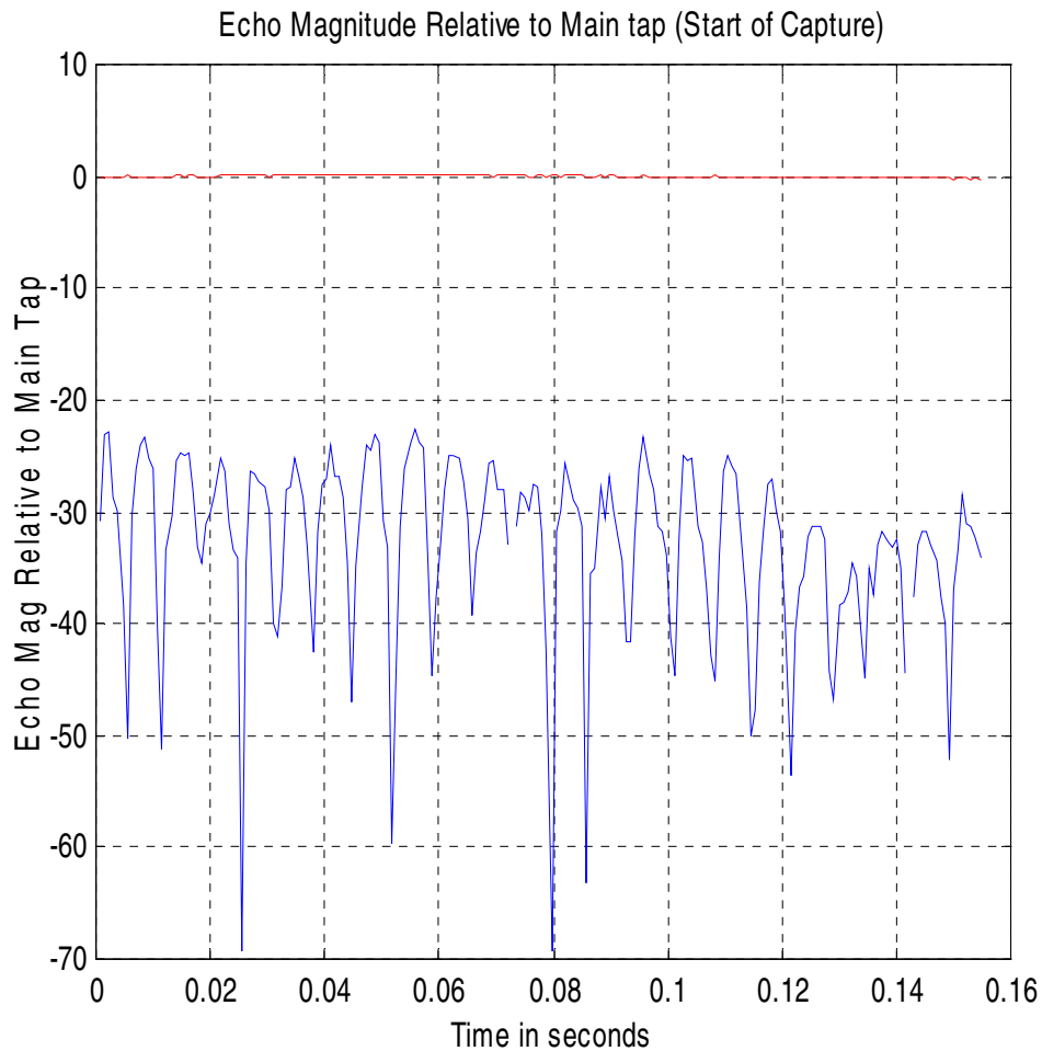
Figure B.9 The 11 \mu\text{s} echo magnitude at the beginning of the capture at indoor site WAS-32/39/01. Doppler frequency is 75 Hz.
