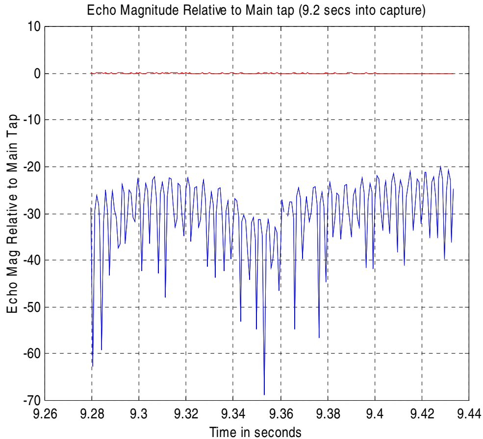
Figure B.15 Echo Magnitude for the 1.75 \mu\text{s} echo relative to the main path, 9.2 seconds into the capture at indoor site WAS-49/36/01. The echo magnitude is -25 dB to -20 dB relative to the main path and has a Doppler frequency of 150 Hz.
