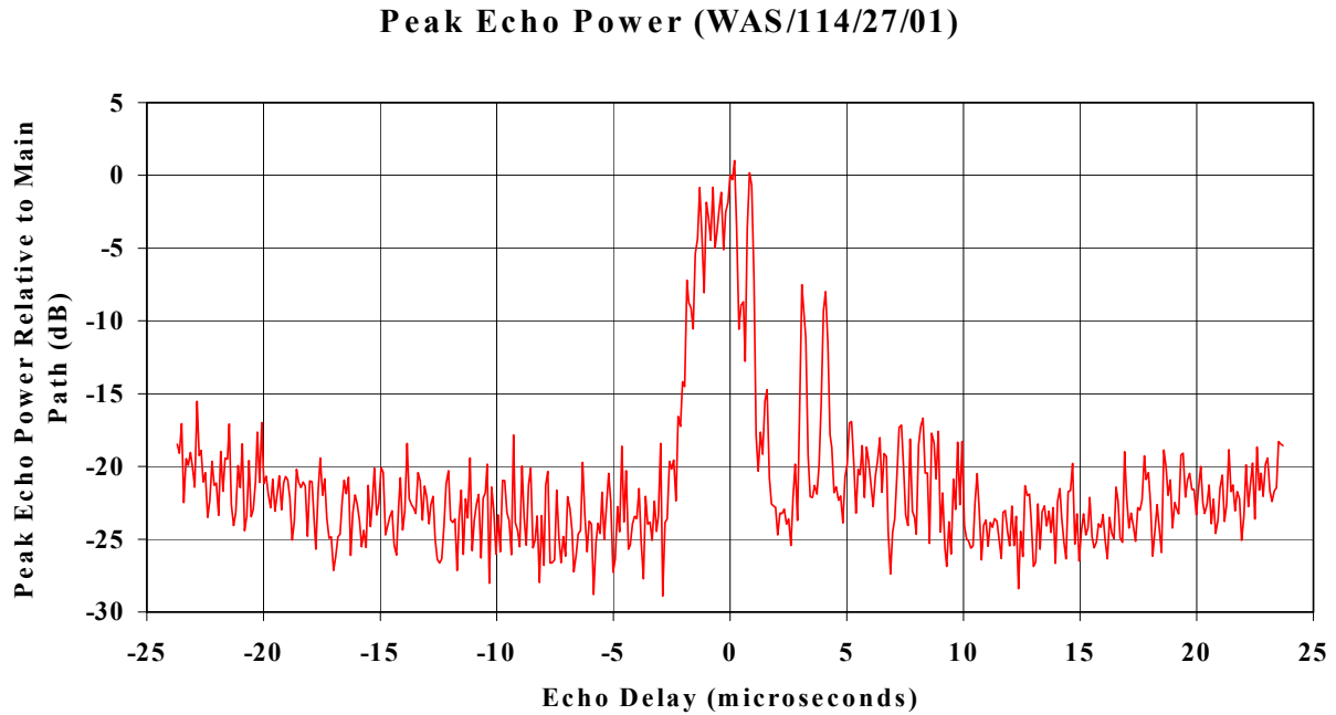
Figure B.24 Peak echo power observed in RF capture WAS/114/27/01
