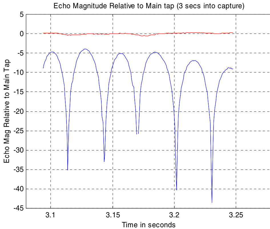
Figure B.13 Echo magnitude for the 1.75 \mu\text{s} echo relative to the main path, 3 seconds into the capture at indoor site WAS-49/36/01. The echo magnitude is -5 dB relative to the main path and has a Doppler frequency of 17 Hz.
