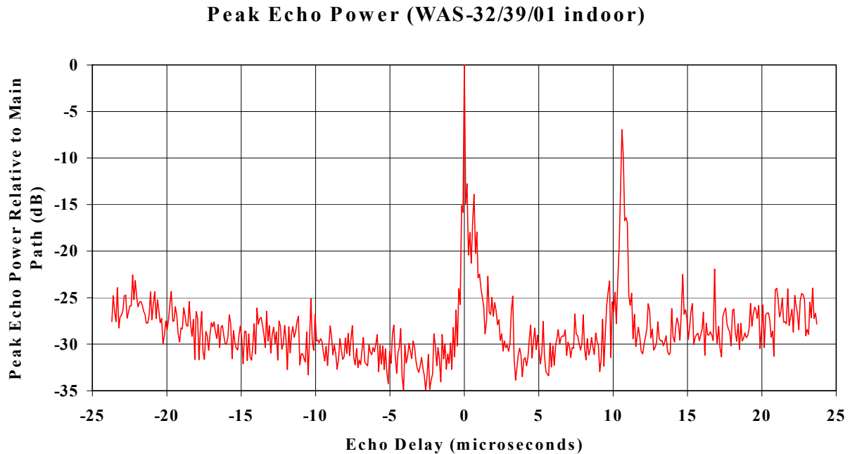
Figure B.8 Peak echo power as a function of echo delay observed for the duration of the RF capture at indoor site WAS-32/39/01.
