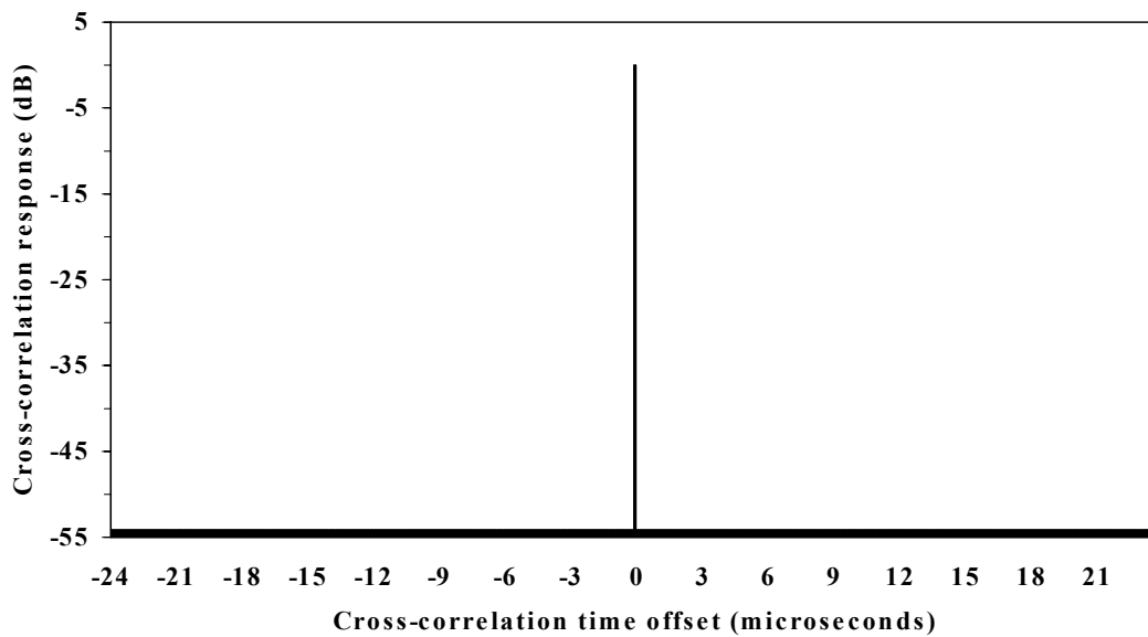
Figure B.2 Cross-correlation of an ideal 8-VSB PN511 sequence showing a single main path at zero microseconds.
