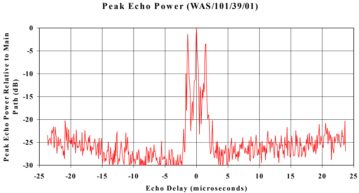
Figure B.25 Peak echo power observed in RF capture WAS/101/39/01
