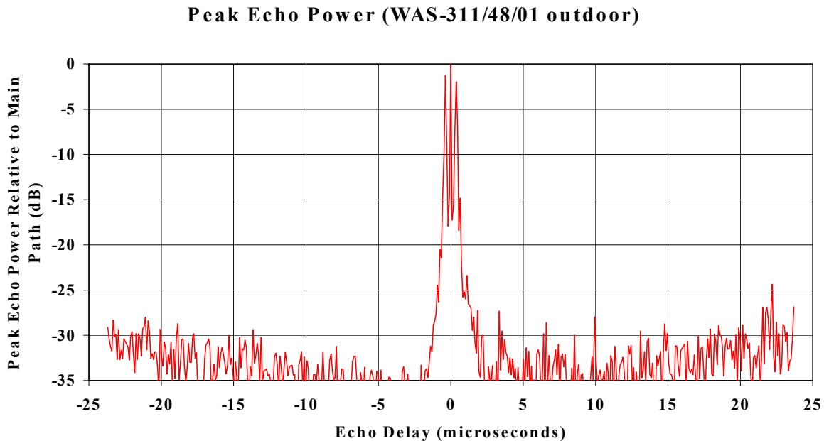
Figure B.21 Peak echo power as a function of echo delay observed for the duration of the RF capture at outdoor site WAS-311/48/01. The evenly spaced close-in echoes peaked at \pm 372 ns indicate that the main path and the echo alternate—a “bobbing” channel.
