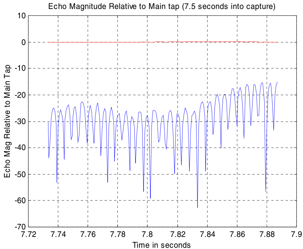
Figure B.14 Echo magnitude for the 1.75 \mu\text{s} echo relative to the main path, 7.5 seconds into the capture at indoor site WAS-49/36/01. The echo magnitude is -25 dB to -15 dB relative to the main path and has a Doppler frequency of 80Hz.
