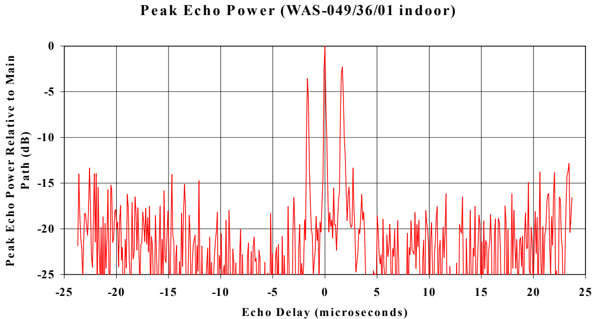
Figure B.11 Peak echo power as a function of echo delay observed for the duration of the RF capture at indoor site WAS-49/36/01. The evenly spaced echoes peaked at \pm 1.67\ \mu\text{s} indicate that the main path and the echo alternate—a “bobbing” channel.
